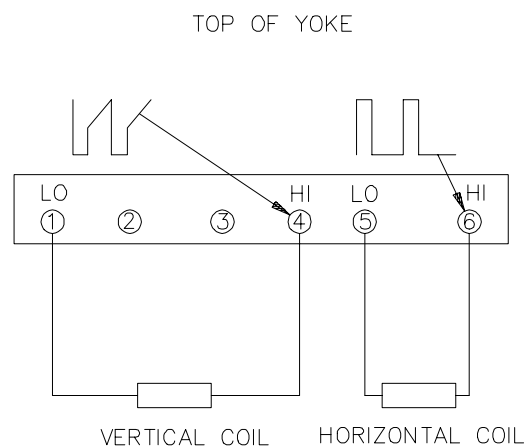
Fig. 1 Connection Diagram for Yoke (As viewed from rear of yoke)
